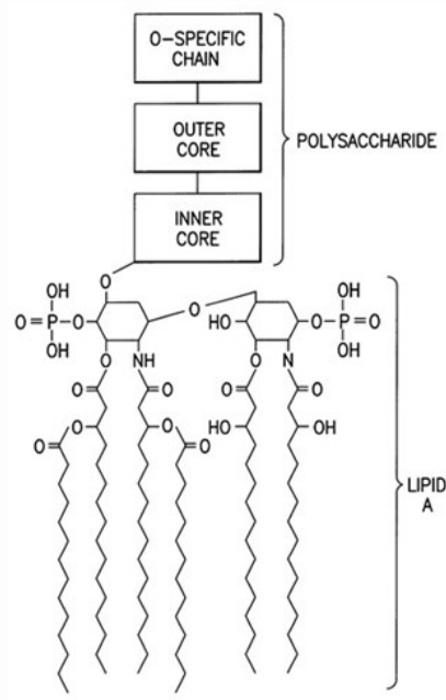
Structure of a lipopolysaccharide
