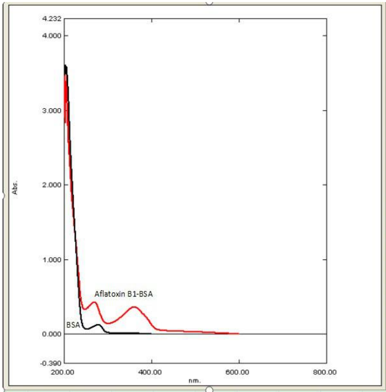
Figure . UV-spectrum
