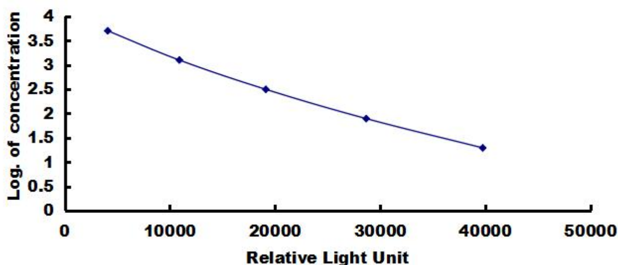
Typical Standard Curve for APP, Human CLIA.
