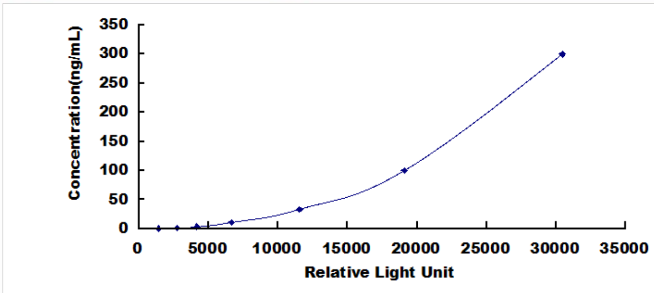
Typical Standard Curve for COMP, Human CLIA.
