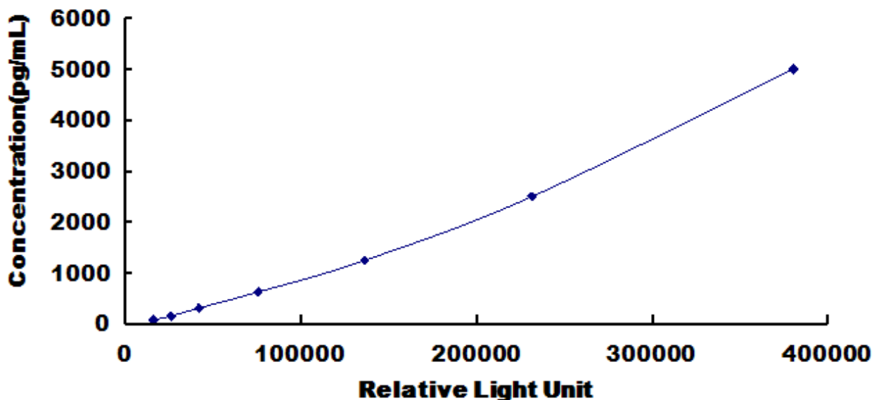
Typical Standard Curve for Rat CKLFSF5 CLIA.
