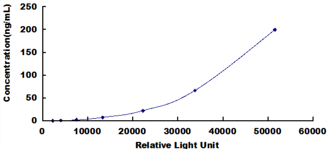
Typical Standard Curve for CST3, Human CLIA.
