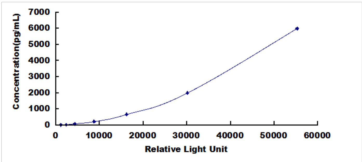
Typical Standard Curve for Erythropoietin, Rat CLIA.
