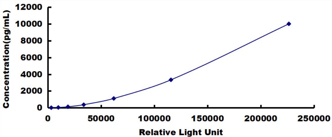
Typical Standard Curve for GLa, Human CLIA.
