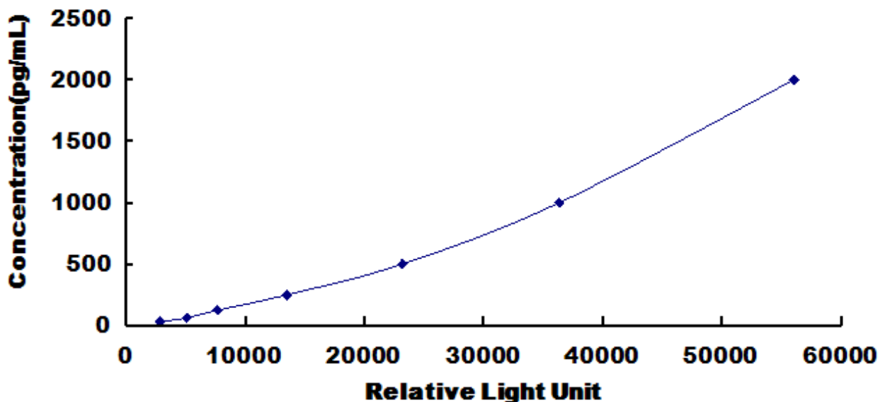
Typical Standard Curve for Mouse IGFL3 CLIA.
