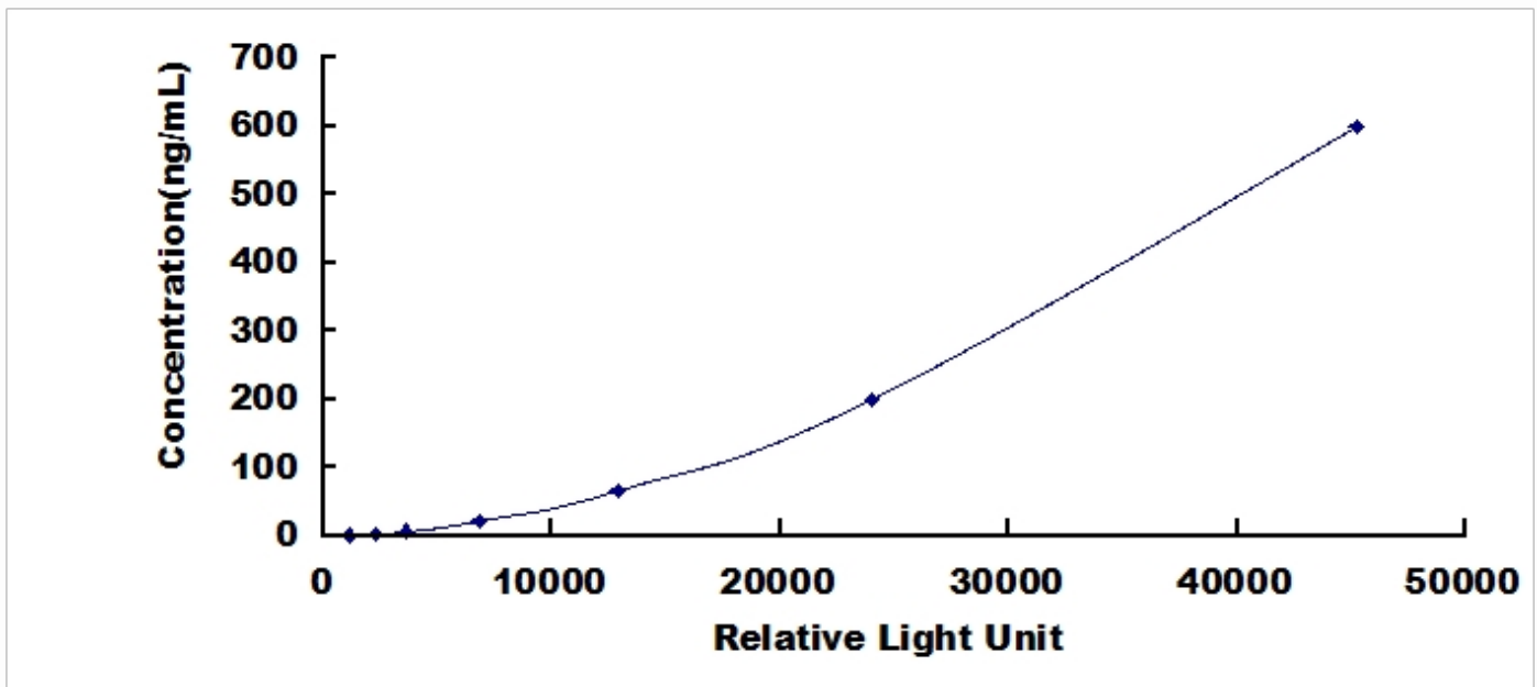
Typical Standard Curve for IGFBP7, Human CLIA.
