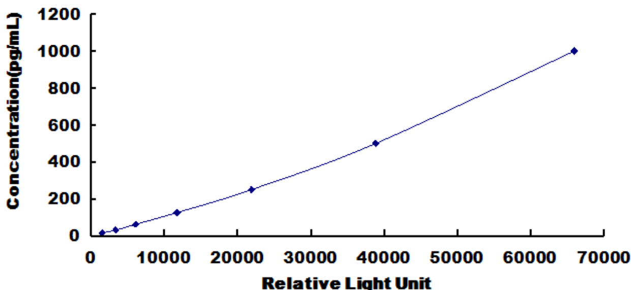
Typical Standard Curve for Human IFNa14 CLIA.
