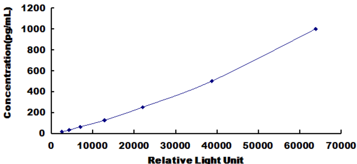
Typical Standard Curve for Human IFNa6 CLIA.
