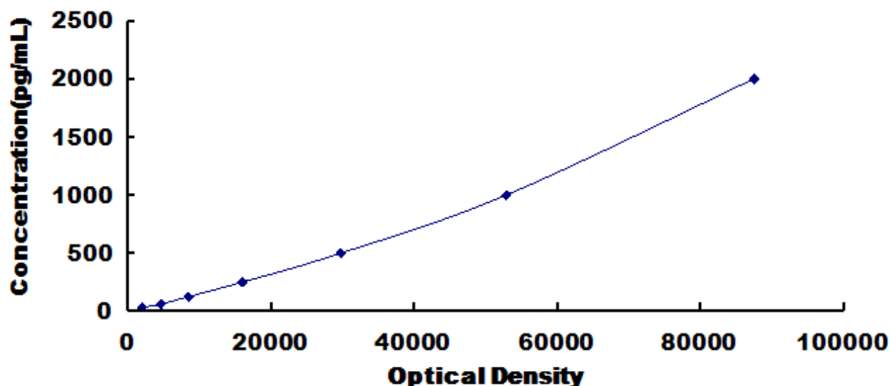
Typical Standard Curve for Human IFI27L1 CLIA.
