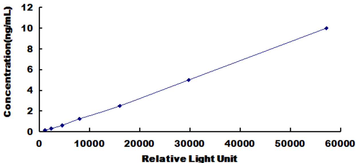
Typical Standard Curve for Mouse IRF2BP1 CLIA.
