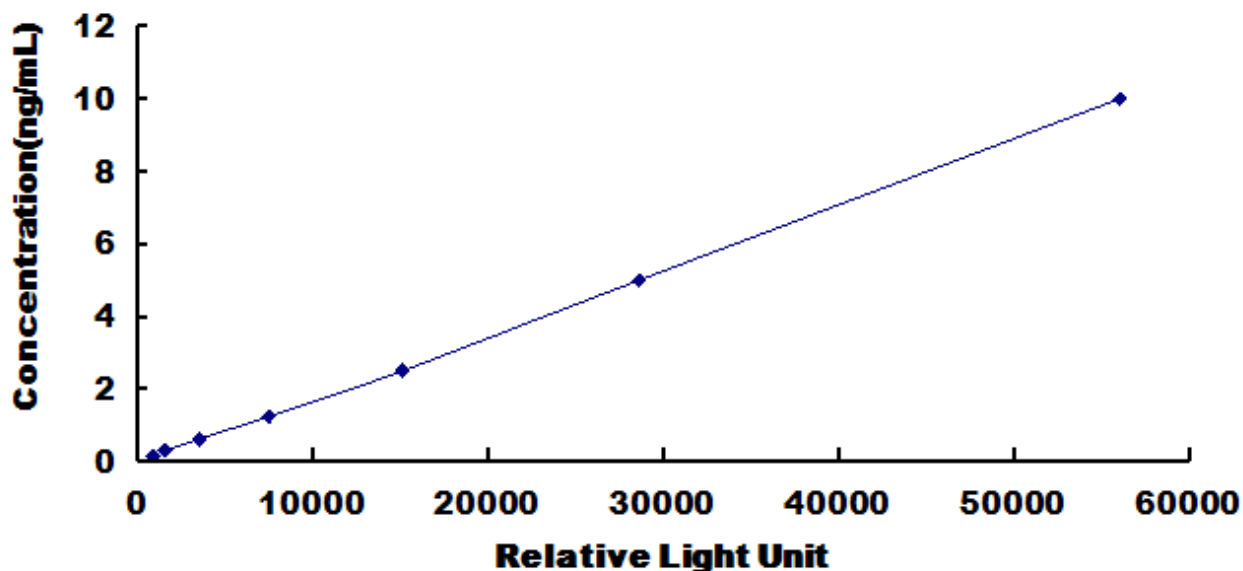
Typical Standard Curve for Rat IRF2BP1 CLIA.
