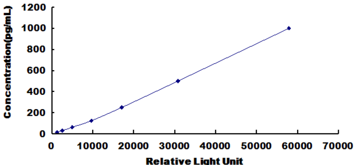
Typical Standard Curve for Human IL1e CLIA.
