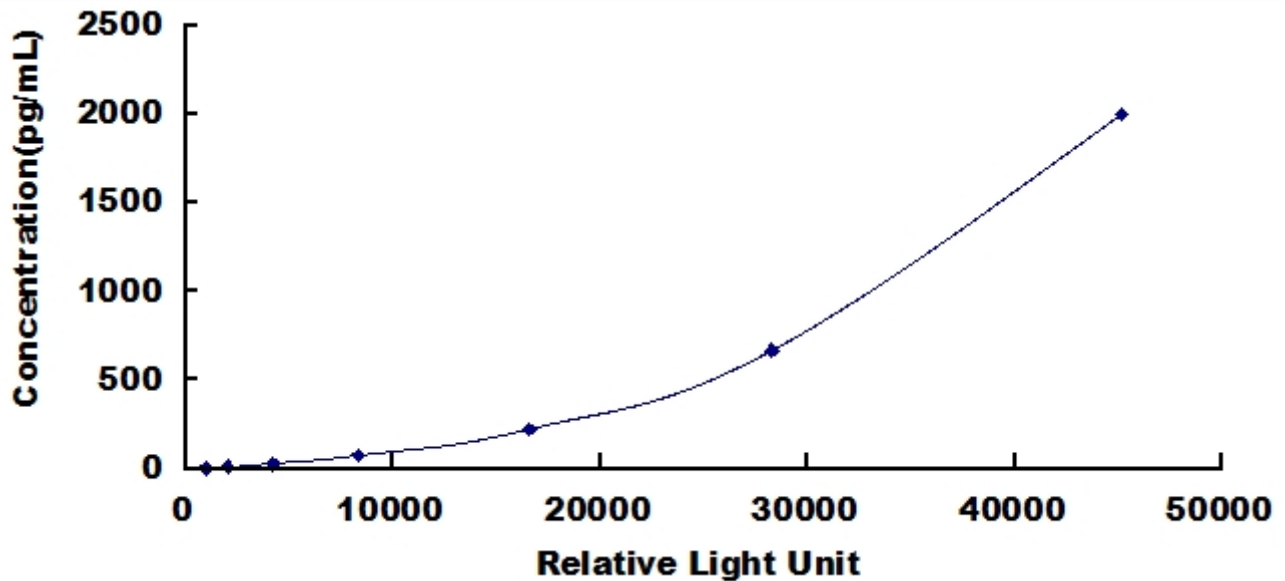
Typical Standard Curve for IL1RAP, Mouse CLIA.
