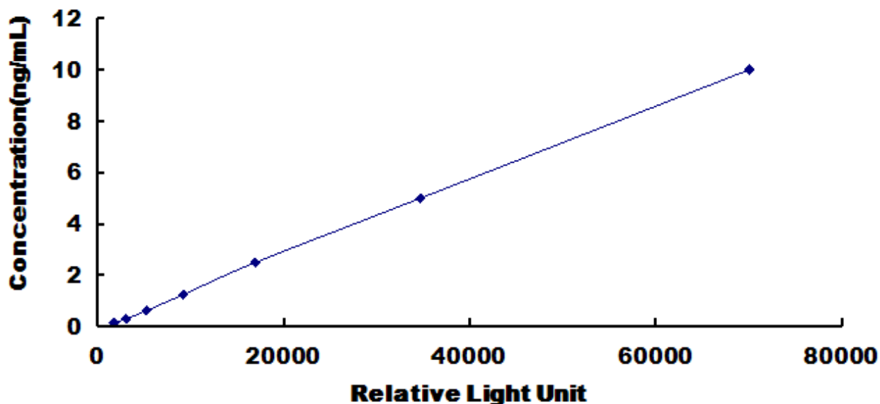
Typical Standard Curve for Mouse IL1RAPL2 CLIA.
