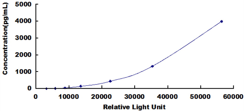
Typical Standard Curve for Myoglobin, Mouse CLIA.
