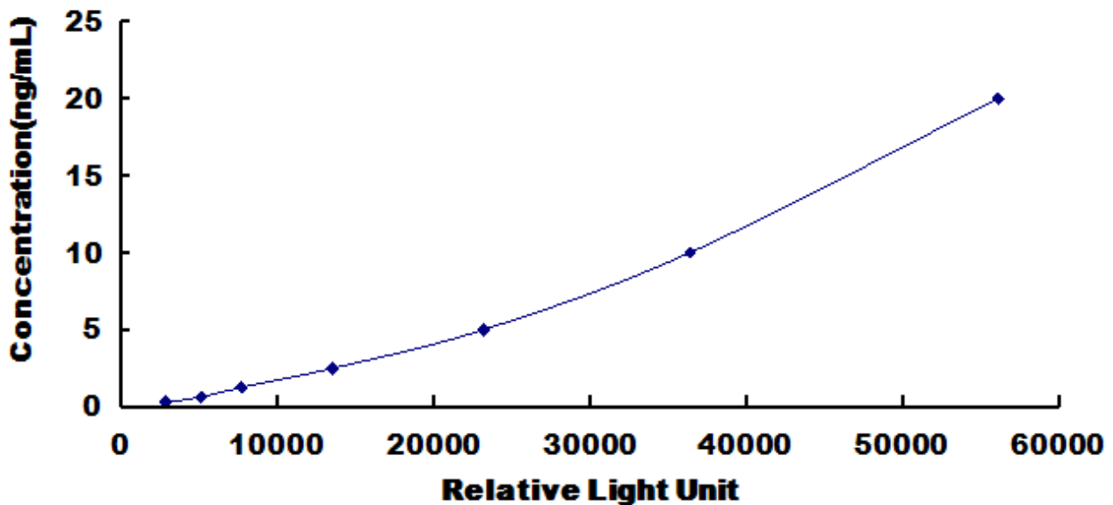
Typical Standard Curve for Human NRP1 CLIA.
