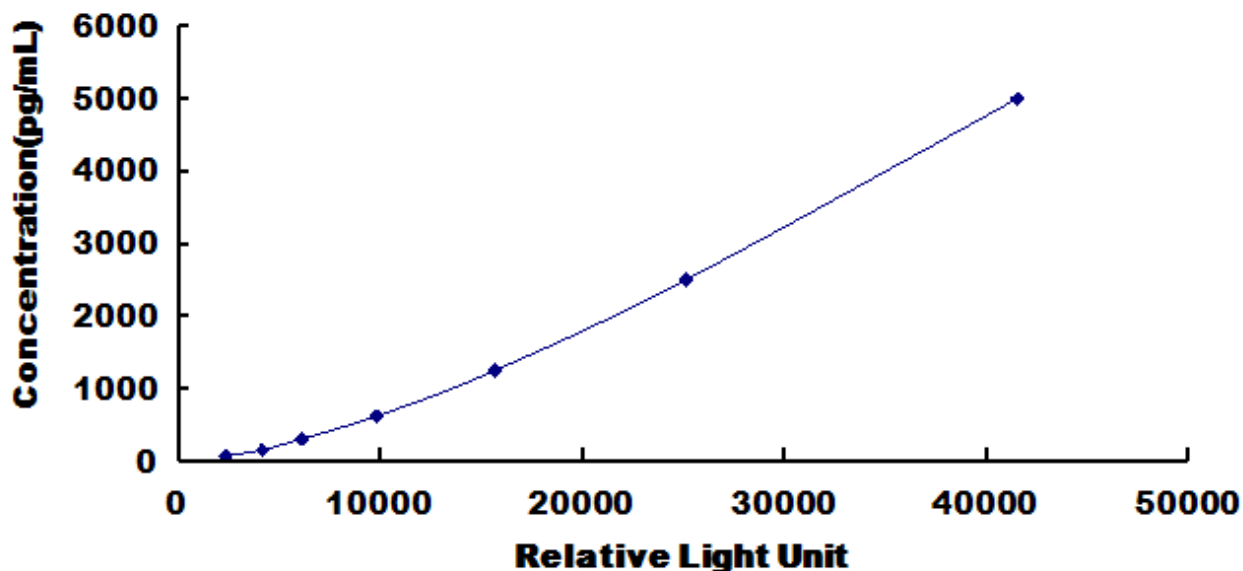
Typical Standard Curve for Mouse PDAP1 CLIA.
