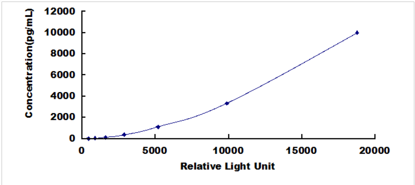
Typical Standard Curve for PSPH, Human CLIA.
