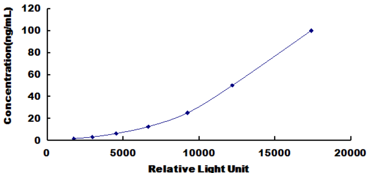
Typical Standard Curve for Rat PEDF CLIA.
