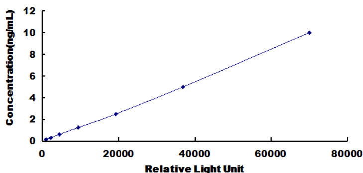
Typical Standard Curve for Human SDF2L1 CLIA.
