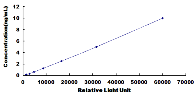
Typical Standard Curve for Rat SDF2L1 CLIA.
