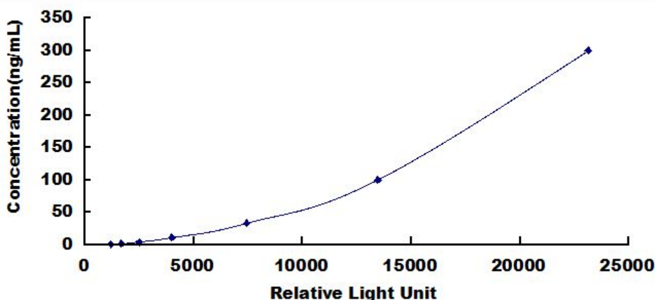
Typical Standard Curve for Teriparatide CLIA.
