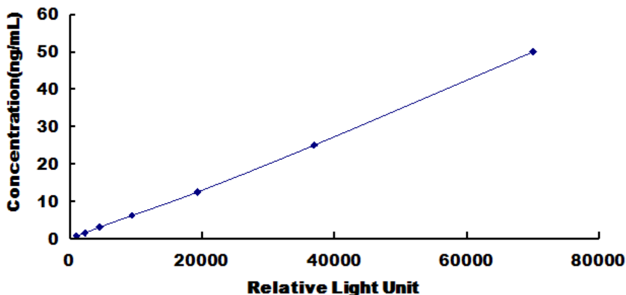
Typical Standard Curve for Bovine TGFβ1 CLIA.
