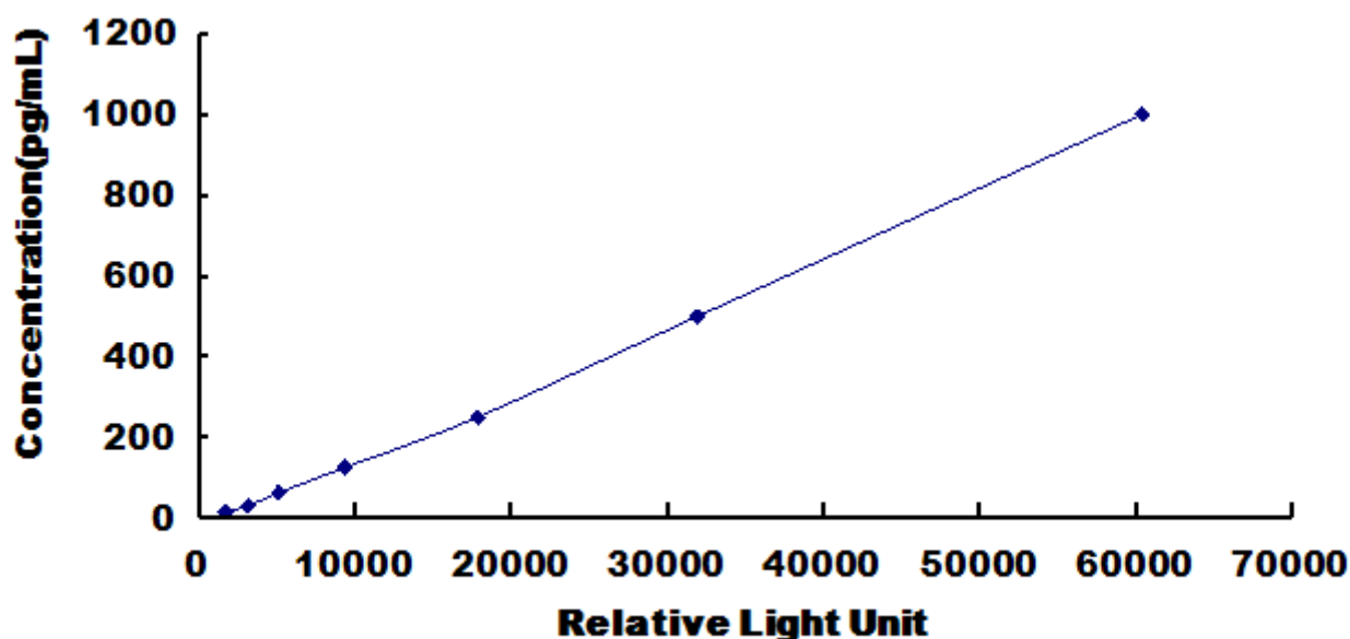
Typical Standard Curve for Porcine TGFβ1 CLIA.
