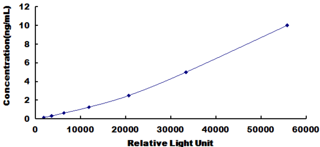
Typical Standard Curve for Human TMED1 CLIA.
