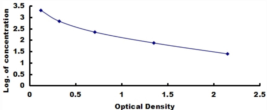
Typical Standard Curve of ELISA Assay for Rat, AngII.
