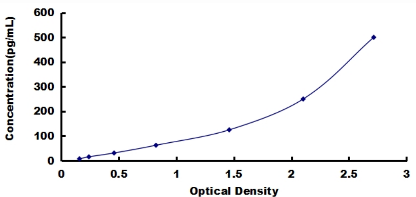
Typical Standard Curve of ELISA Assay for Human IFNa.
