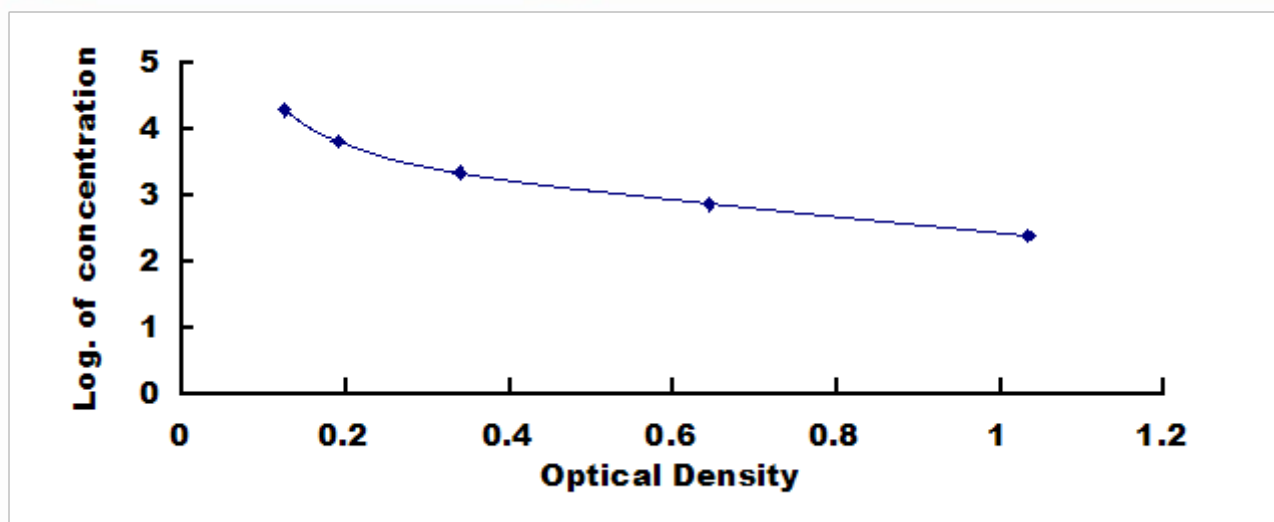
Typical Standard Curve for 17-OHP ELISA.
