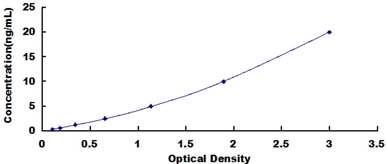
Typical Standard Curve for OASL, Human ELISA.
