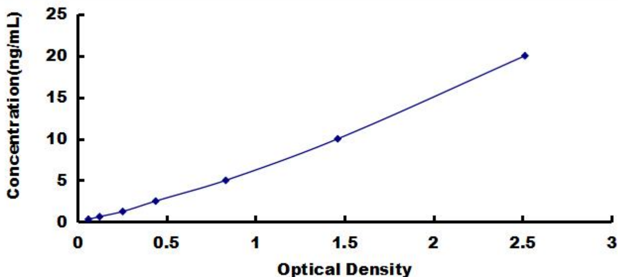
Typical Standard Curve for NT5C3, Human ELISA.
