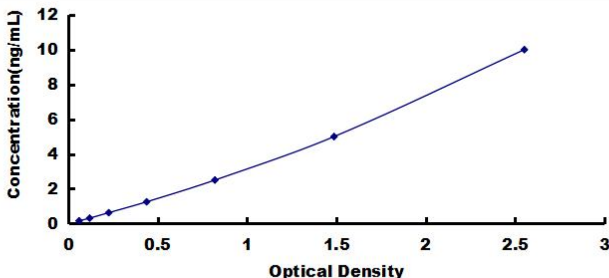
Typical Standard Curve for ADAM9, Rat ELISA.
