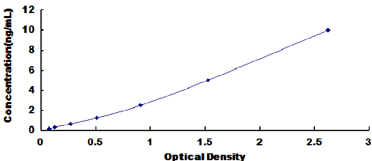
Typical Standard Curve for ATP1a1, Rat ELISA.
