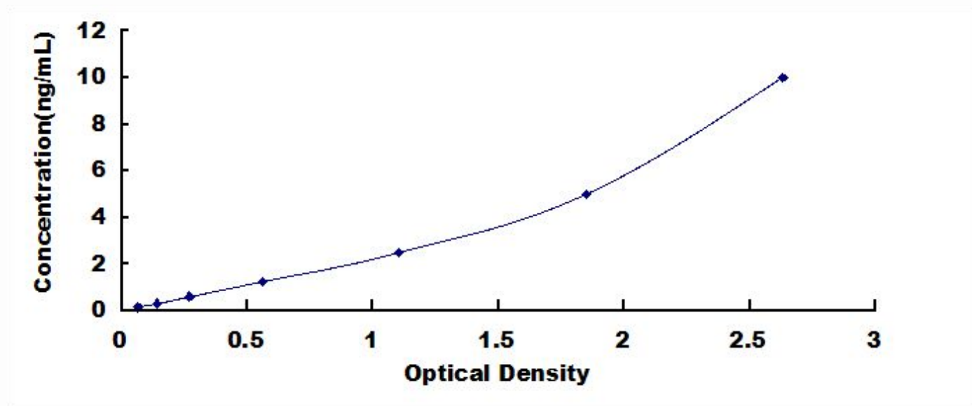
Typical Standard Curve for ACTR3, Human ELISA.
