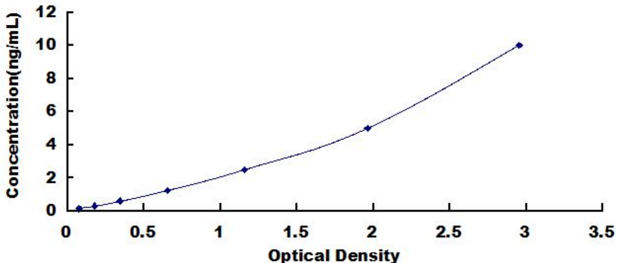
Typical Standard Curve for ATF4, Mouse ELISA.
