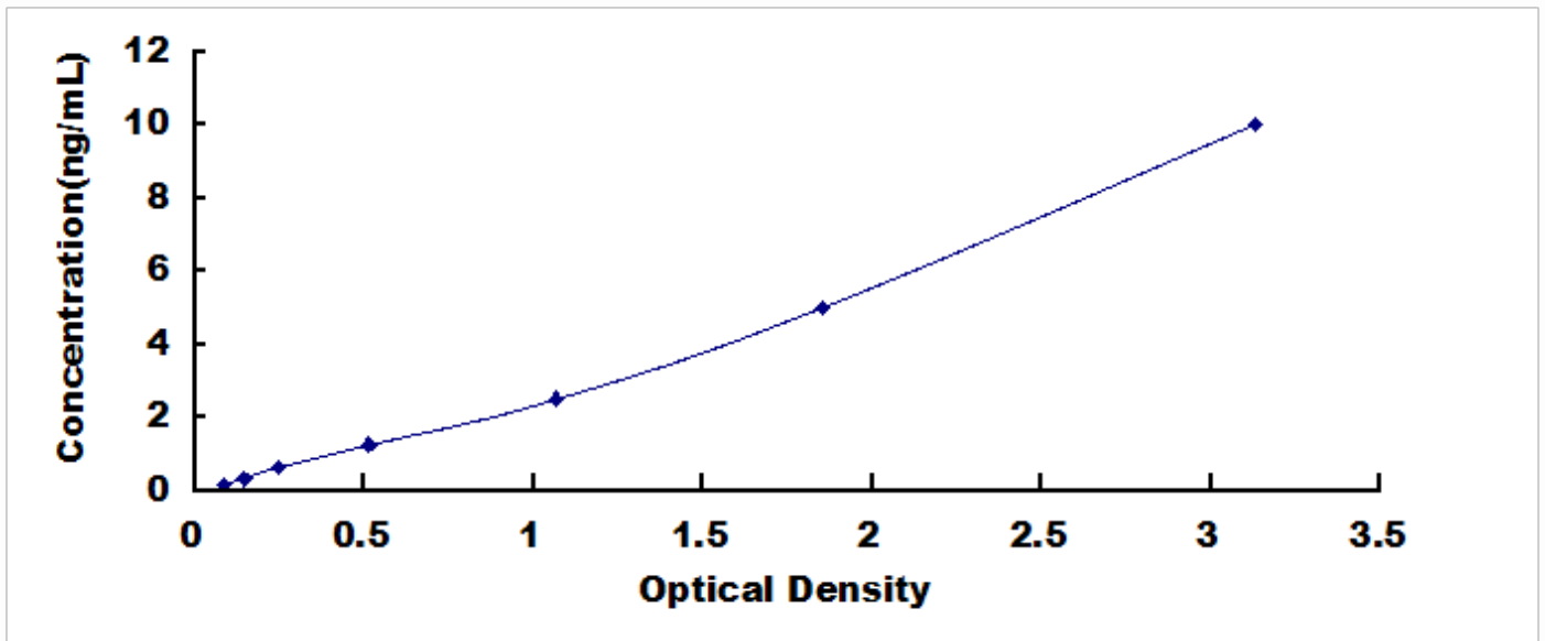
Typical Standard Curve for AIP, Human ELISA.
