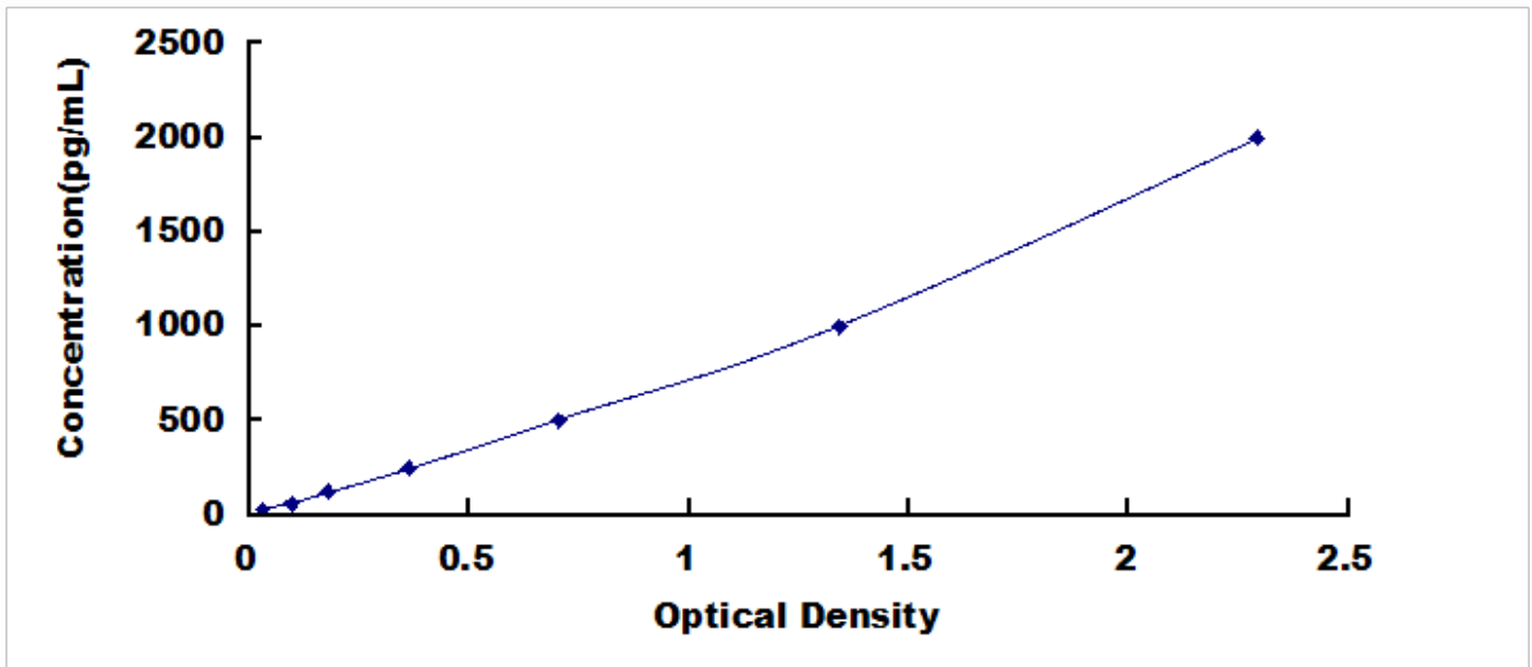
Typical Standard Curve for BMP4 ELISA.
