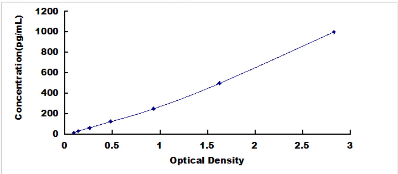
Typical Standard Curve for CDH16, Human ELISA.
