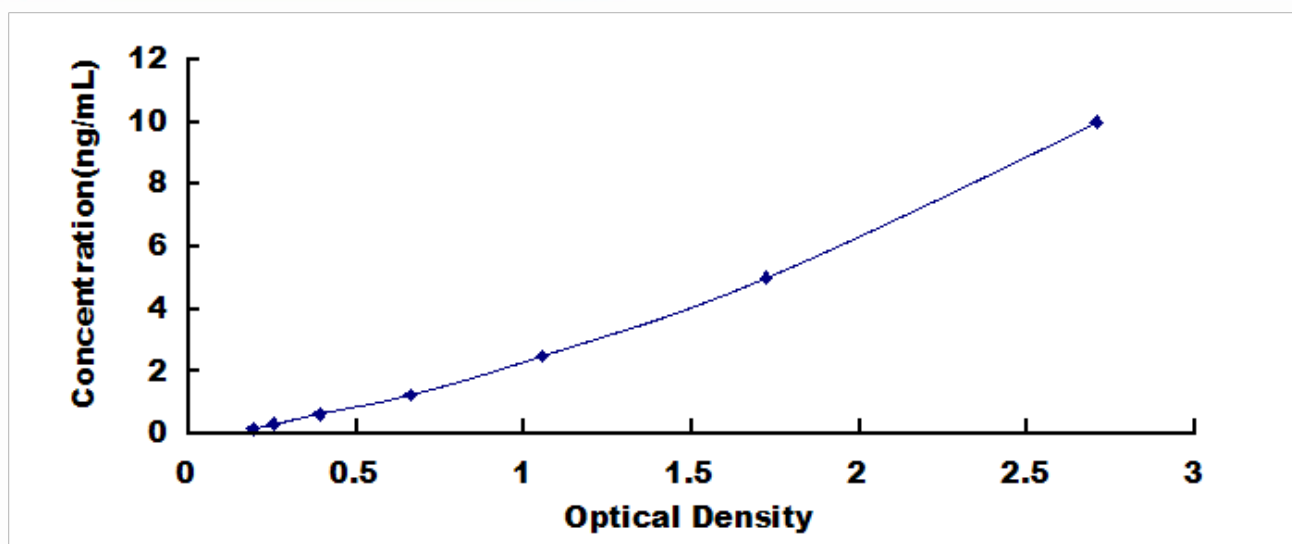
Typical Standard Curve for CA2, Human ELISA.
