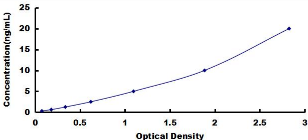
Typical Standard Curve for CNDP2, Mouse ELISA.
