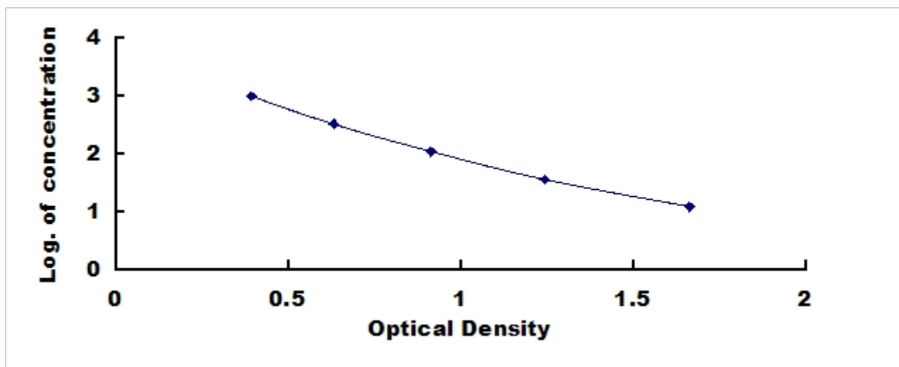
Typical Standard Curve for CCK8, Human ELISA.
