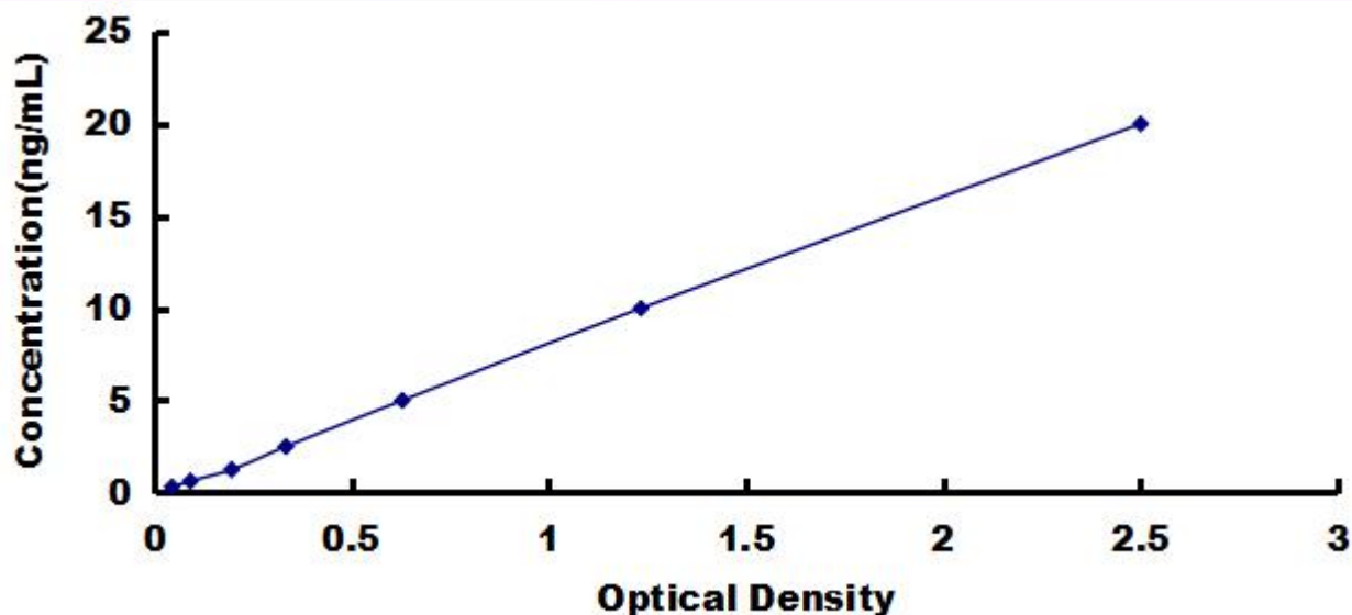
Typical Standard Curve for COL1a2, Canine ELISA.
