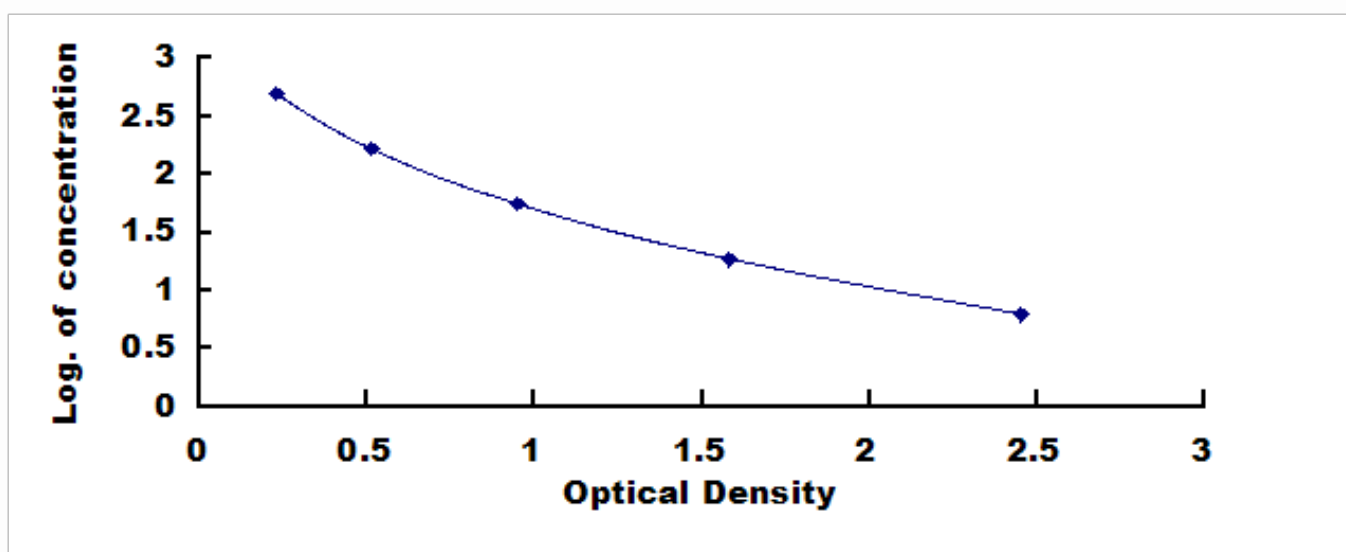
Typical Standard Curve for Corticosterone ELISA.
