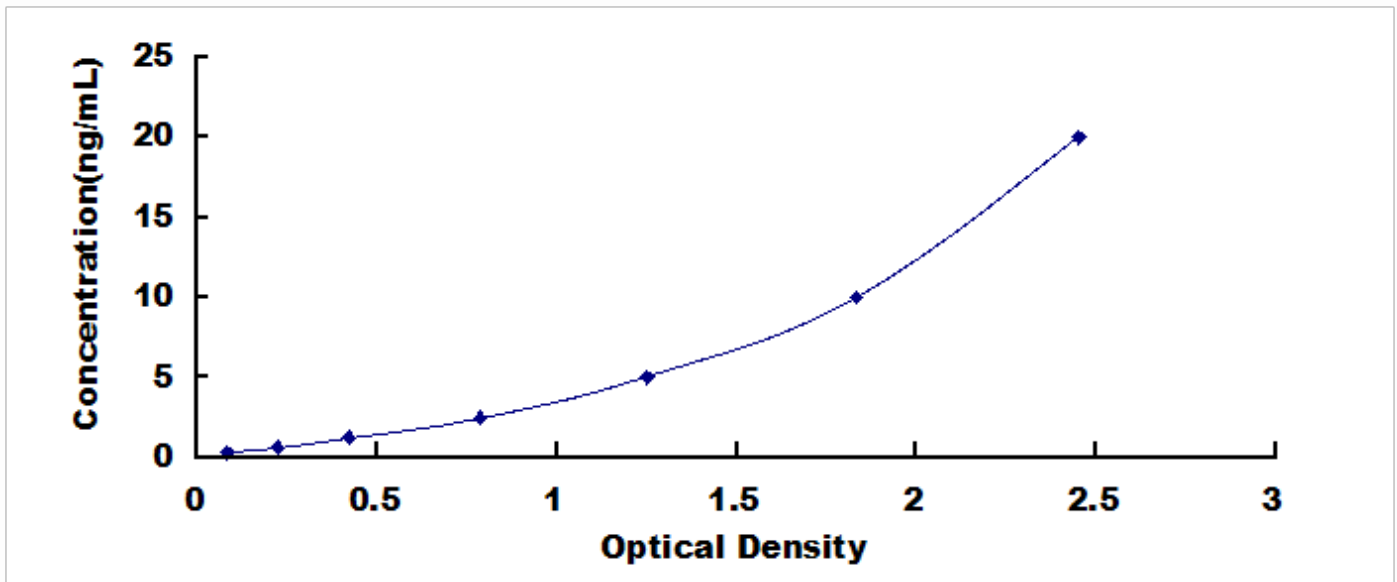
Typical Standard Curve for CDK4, Human ELISA.
