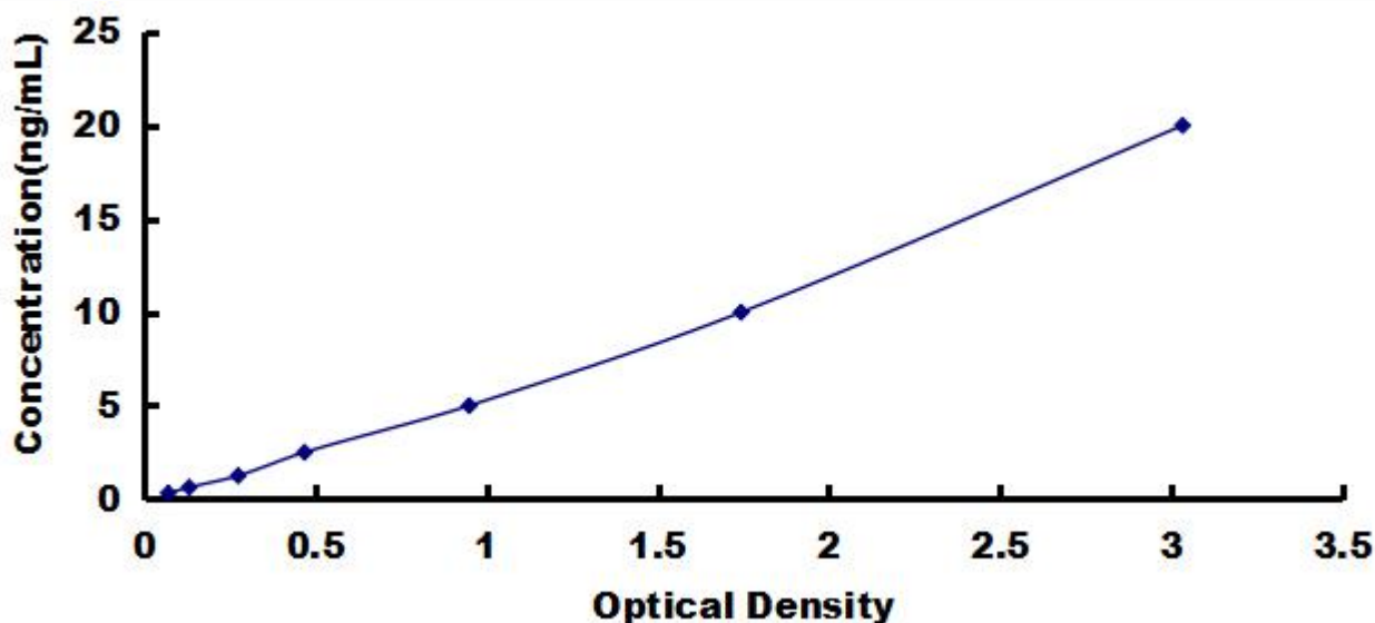
Typical Standard Curve for CDK8, Mouse ELISA.
