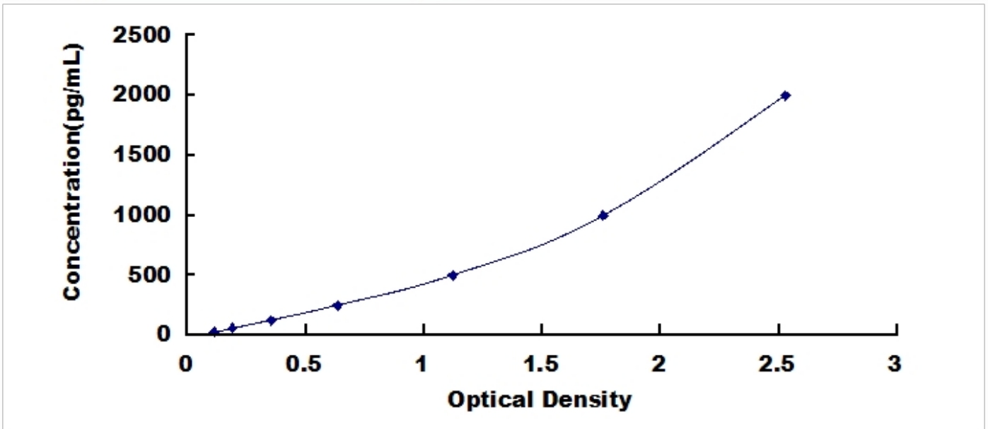
Typical Standard Curve for DAO, Mouse ELISA.
