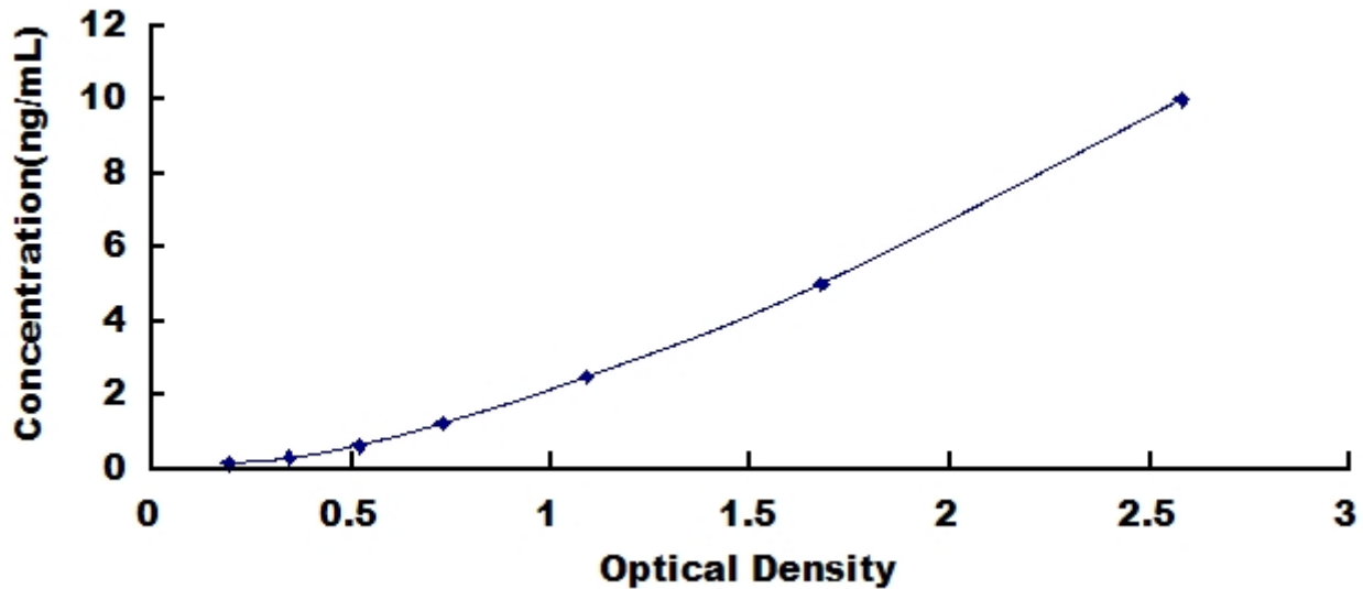
Typical Standard Curve for DUSP6, Mouse ELISA.
